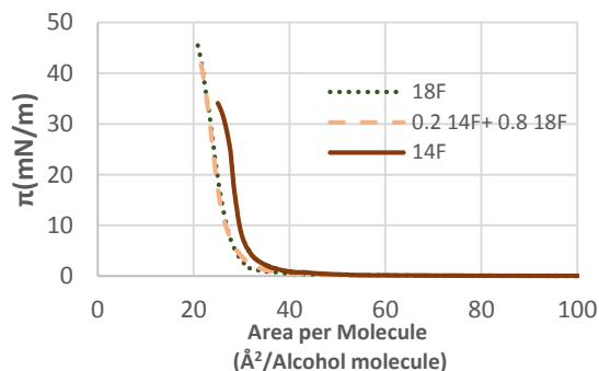
Figure 8 - Langmuir balance Isotherm of 18F and 14F, pure and mixtures, at 293.15K.
