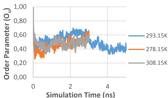
Figure 19 - Evolution of the order parameter of 14F at different temperatures in time, 278.15K, 293.15K, 308.15K.
