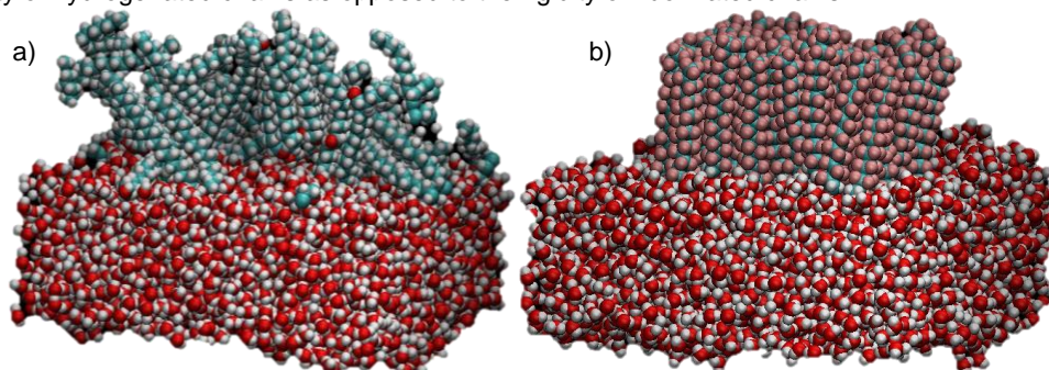
Figure 15 – a) 18H and b) 18F, above water after 25ps of simulation time.
