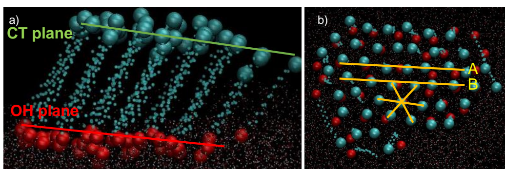
Figure 16 – a) Lateral and b) vertical projections of 18F. Red spheres represent oxygen atoms of OH groups. Blue spheres represent the carbon atoms terminal CH 3 groups.
