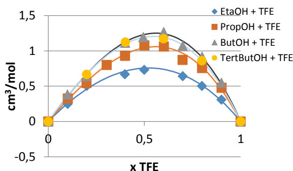
Figure 3 – Excess molar volume of hydrogenated alcohols and TFE mixtures. Points represent experimental results and the solid lines the Redlich-Kister equation.
