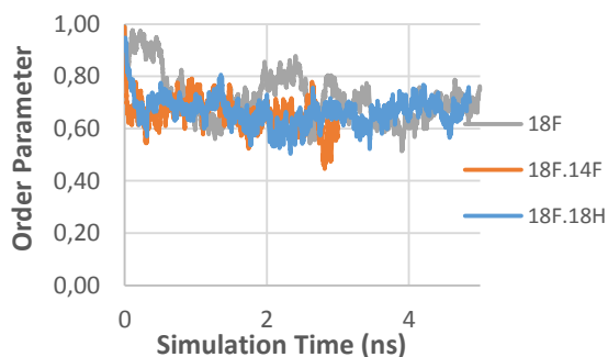
Figure 21 - Order Parameter as a function of time for both mixtures, 18F-14F and 18F-18H.
