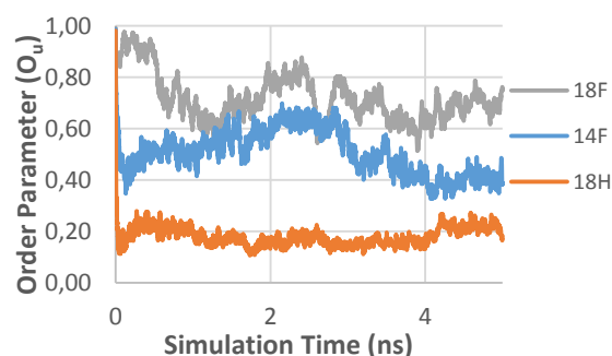
Figure 17 – Evolution of order parameter of Alcohols (18F, 14F, 18H) molecules in time.
