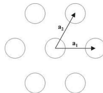
Figure 22 – Hexagonal Lattice.
