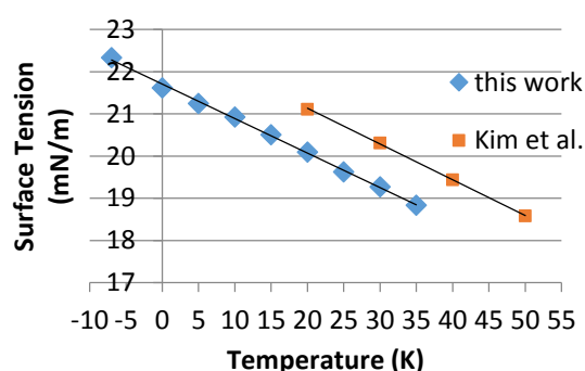
Figure 1 - Surface Tension of TFE as a function of temperature.
