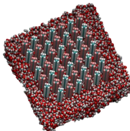
Figure 20 - Initial configuration of 18F + 18H mixture.
