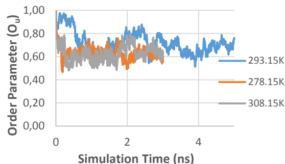
Figure 18 - Evolution of the order parameter of 18F at different temperatures in time, 278.15K, 293.15K, 308.15K.
