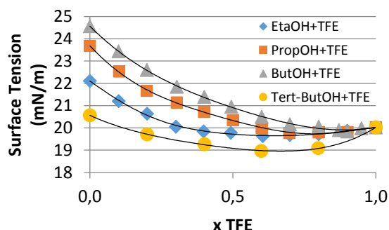
Figure 2 - Surface Tension of mixtures of hydrocarbon and fluorinated alcohols as a function of composition at 293.15K.
