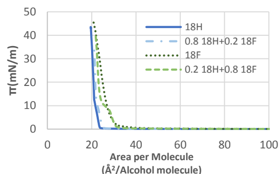
Figure 4 - Langmuir Isotherms of 18F and 18H, pure and mixtures, at 293.15K.
