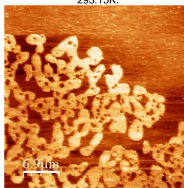
Figure 9 - AFM scan of pure 14F at 70\text{\AA}^2/\text{molecule} – topography contrast.
