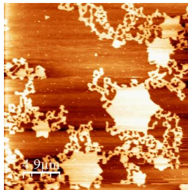
Figure 10 - AFM scan of mixture between 18F and 14F (0.8-0.2) at 80 \text{\AA}^2 /molecule – topography contrast.
