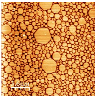
Figure 12 - AFM scan of pure 18F at 30 \text{\AA}^2 /molecule and 5mN/m and 308.15K – topography contrast.
