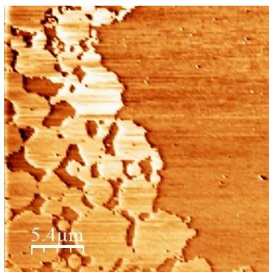
Figure 14 - AFM scan of pure 14F at 32 \text{\AA}^2 /molecule and 5mN/m 278.15K – phase contrast.
