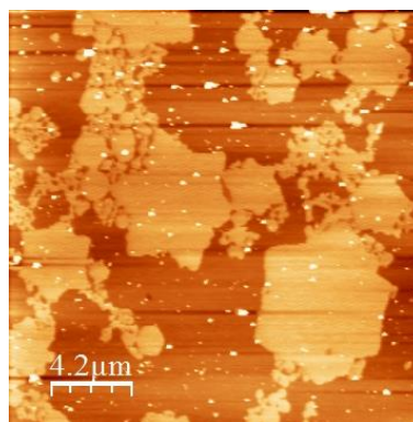
Figure 7 – AFM scan of pure 18F at 85\text{\AA}^2/\text{molecule} - topography contrast.
